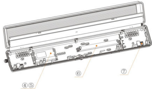
全塑防爆LED应急条形灯 CZ0866/2 × LED 30W□ YJ Full plastic explosion-proof LED (emergency) linear light fittings
